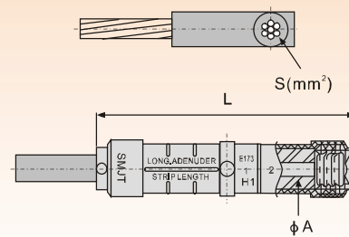
cutaway view of joint pipe
