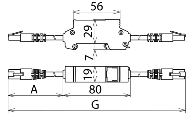
Dimension drawing DPA M CAT6 RJ45H 48
