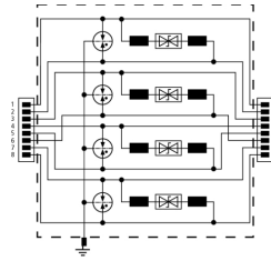
Basic circuit diagram DPA M CAT6 RJ45H 48
