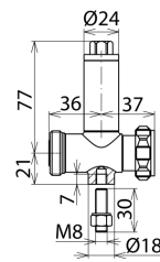
Dimension drawing DGA LG 7 16 X
