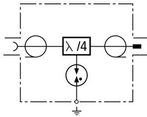
Basic circuit diagram DGA LG 7 16 X
