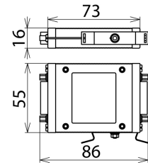
Dimension drawing USD 25 V24 HS S B
