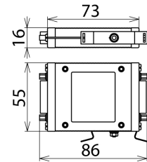
Dimension drawing USD 9 V24 B
