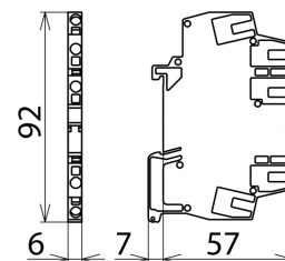
Dimension drawing DCO RK E 48
