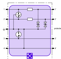
Basic circuit diagram BXT ML2 BE S 48
