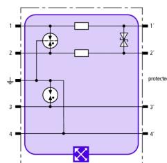
Basic circuit diagram BXT ML2 BD S 12
