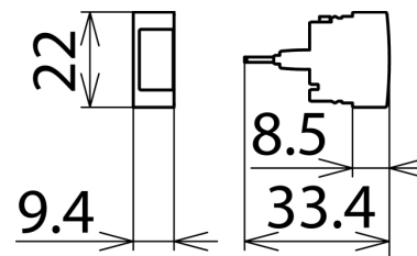
Dimension drawing DRL RE 60
