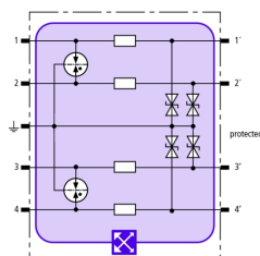
Basic circuit diagram BXT ML4 BE 24
