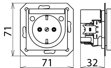
Dimension drawing NSM PRO AZ
