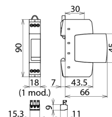
Dimension drawing DR M 2P 75 FM
