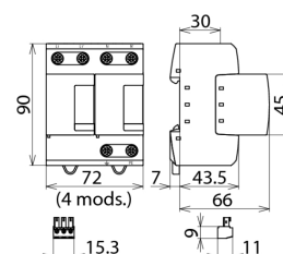
Dimension drawing DV M TN 255 FM
