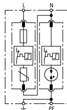
Basic circuit diagram DG M TT 2P CI 275
