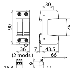
Dimension drawing DG M TN CI 275
